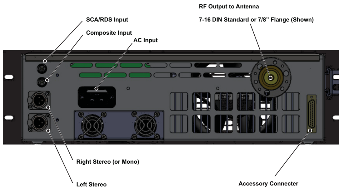
Figure 3-1. FM1050ES Rear-Panel Connectors
