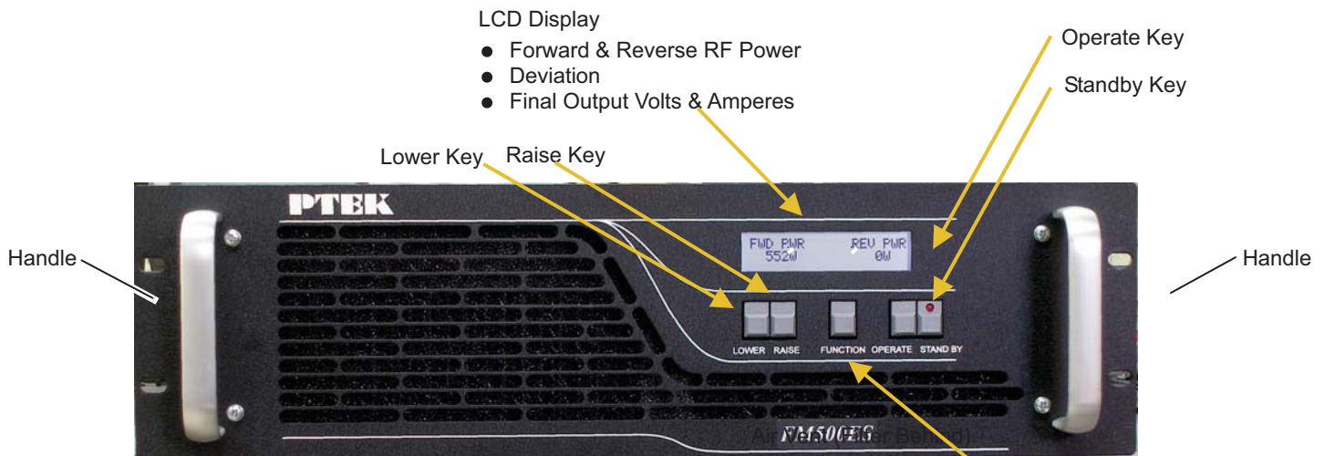
Figure 1-3. FM1050ES Front Panel
