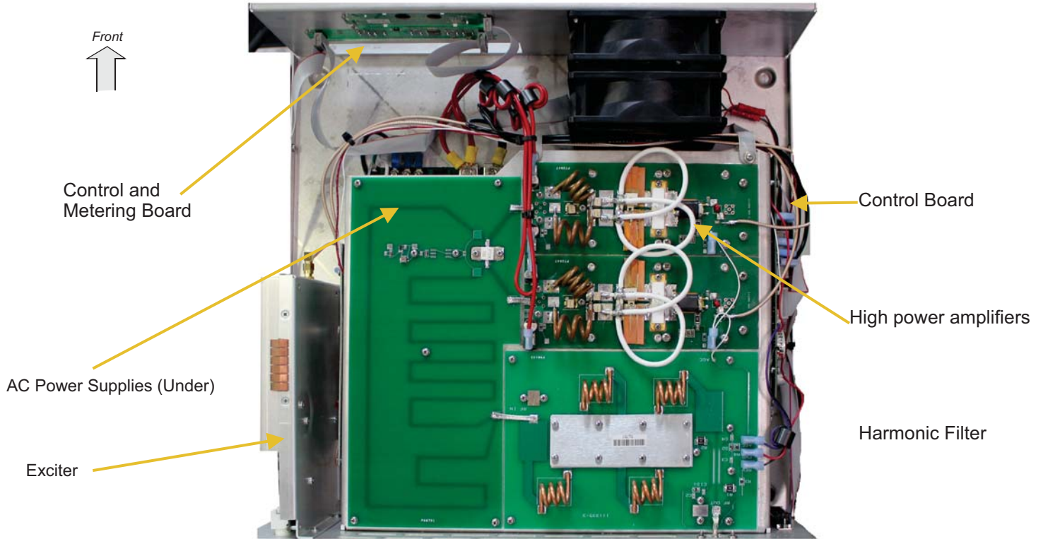
A FM1050ES Top View (Cover Off)
